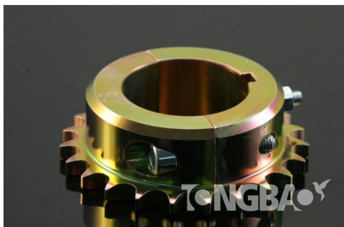
23T #428 Sprocket, Inner Diameter:50mm,Keyway width:8mm
