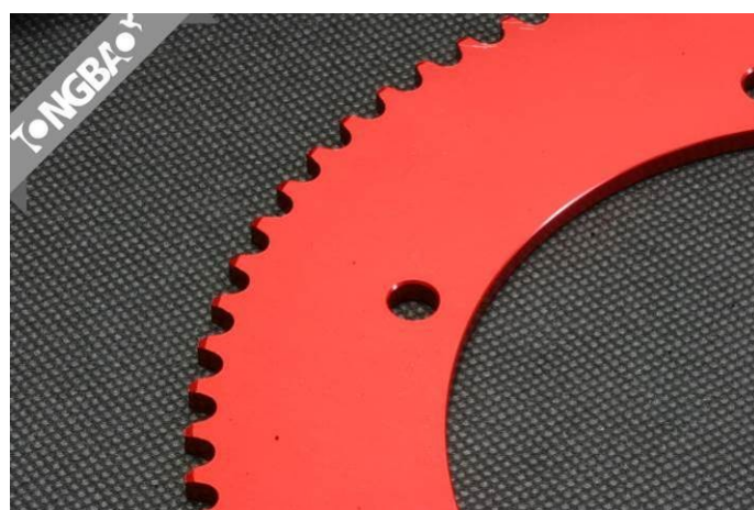
Traditional Red Anodized #35 Aluminum Split Sprocket
